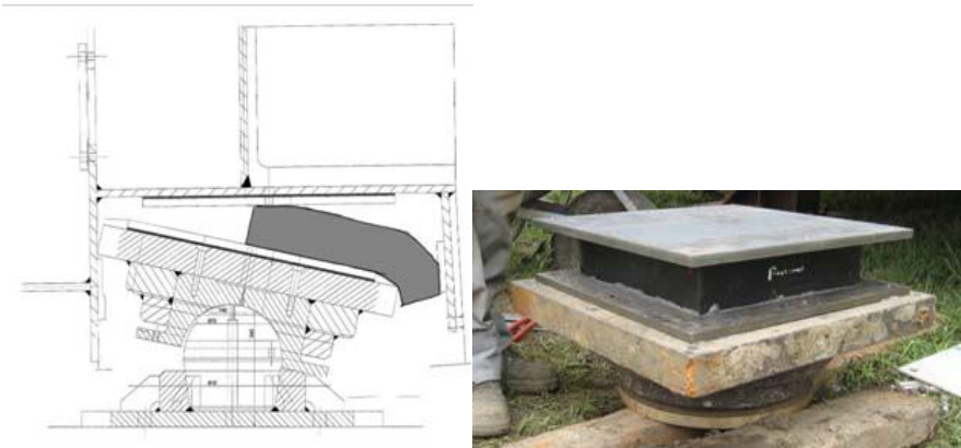
Figure 1: The lower support with the pintle (rotation around vertical axis) and a neoprene support (as in bridge) to allow heeling and a small horizontal displacement
